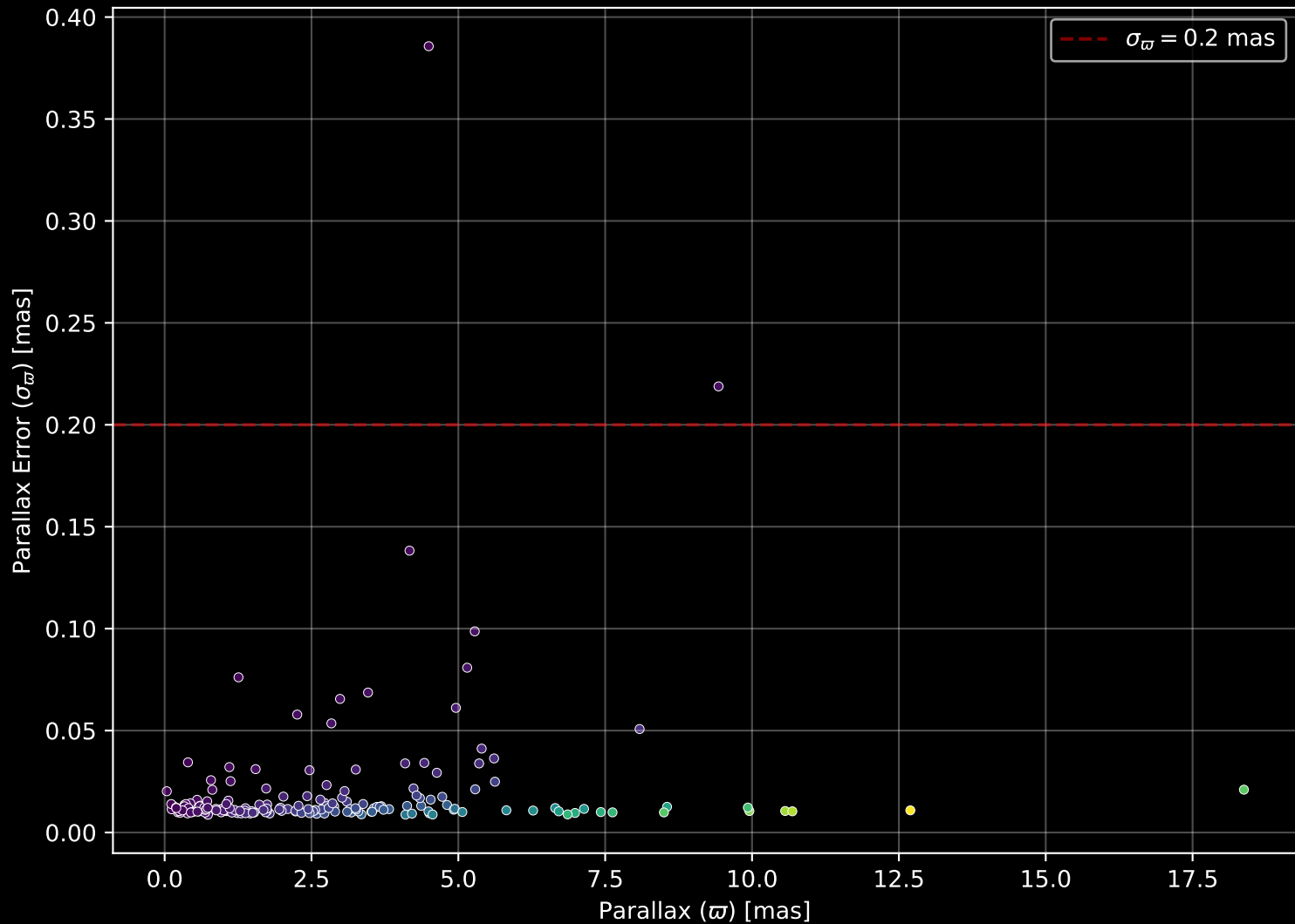
APOGEE DR17 Field: [273-28-O_TESS] Parallax Quality (n= 181)
