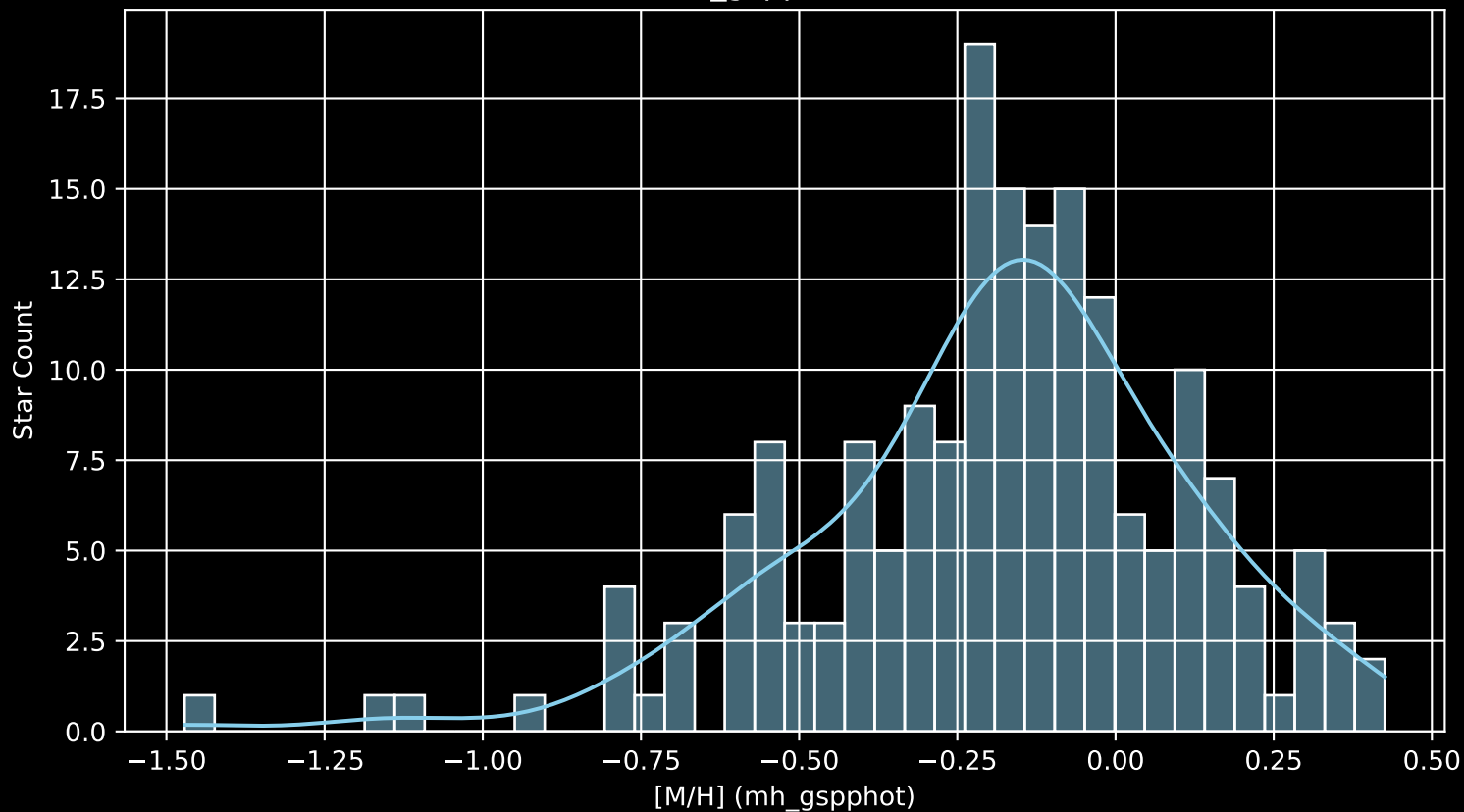
APOGEE DR17 Field: [273-28-O_TESS [M/H] (mh_gspphot) (n= 180)
