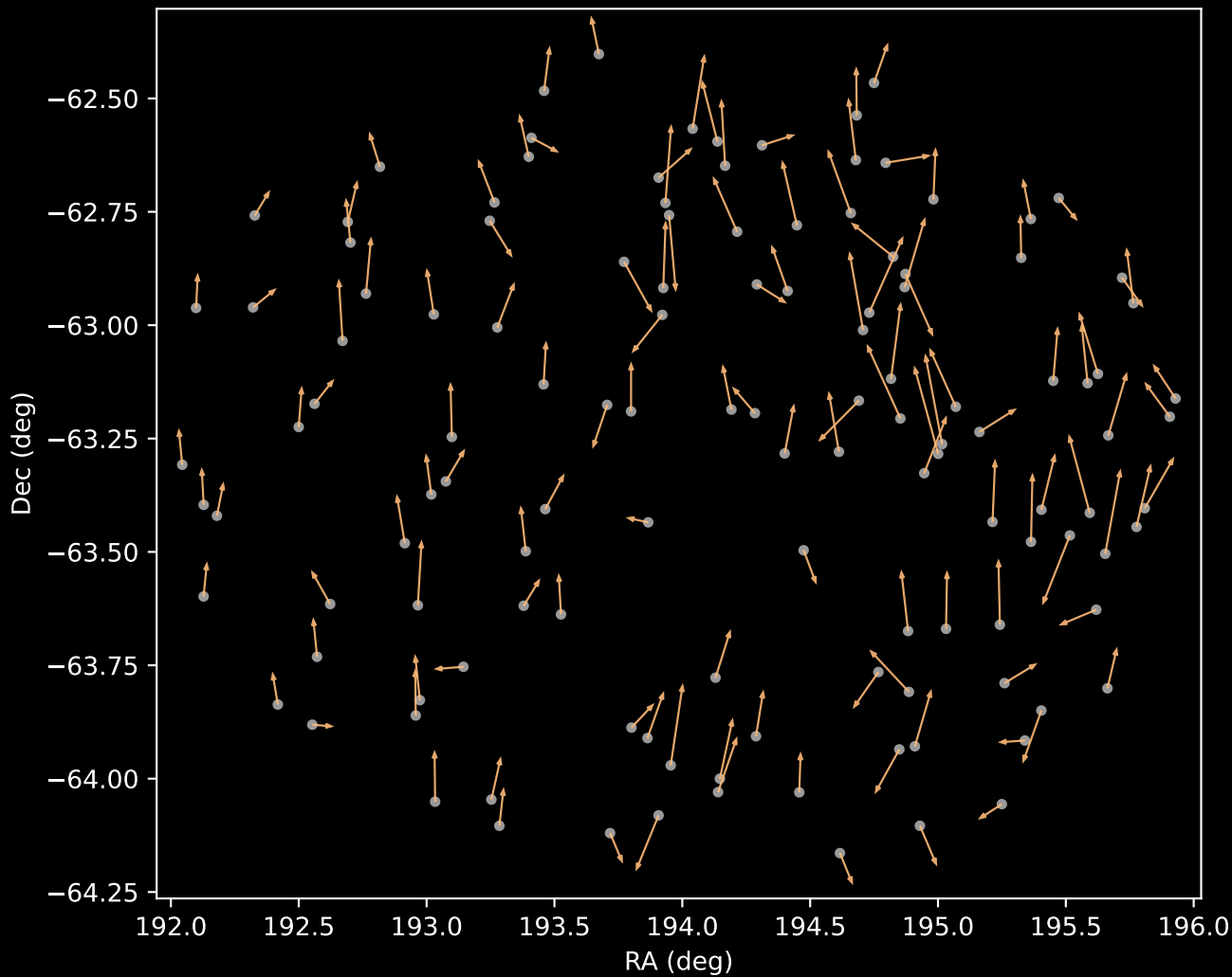
APOGEE DR17 Cluster 3 Proper Motion Vectors (n=127)
