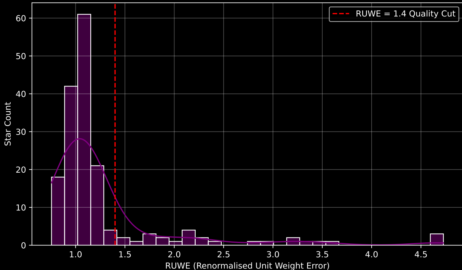
GAPOGEE DR17 Field [273-28-O_TESS] RUWE Distribution (n= 172)
