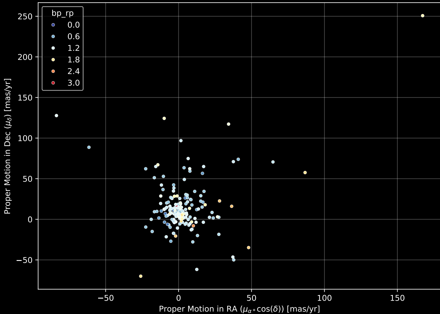
APOGEE DR17 Field: [273-28-O_TESS] Proper Motion Diagram (n= 181)
